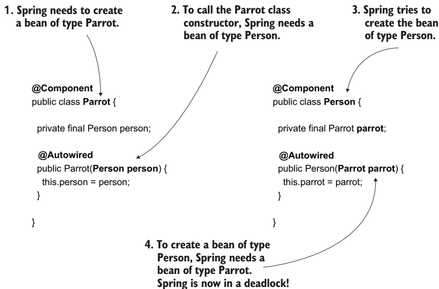
Figure 3.11 A circular dependency. Spring needs to create a bean of type Parrot. But because Parrot has as a dependency a Person, Spring needs first to create a Person. However, to create a Person, Spring already needs to have built a Parrot. Spring is now in a deadlock. It cannot create a Parrot because it needs a Person, and it cannot create a Person because it needs a Parrot.
