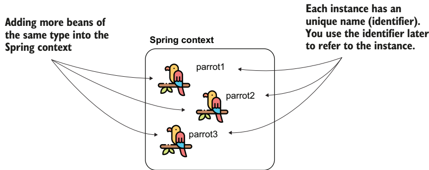
Figure 2.11 You can add more beans of the same type to the Spring context by using multiple methods annotated with @Bean . Each instance will have a unique identifier. To refer to them afterward, you'll need to use the beans' identifiers.
