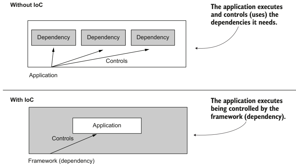
Figure 3.8 An application that’s not using the IoC principle controls the execution and makes use of various dependencies. An application using the IoC principle allows a dependency to control its execution. The DI is such an example of control. The framework (a dependency) sets a value into a field of an object of the app.
