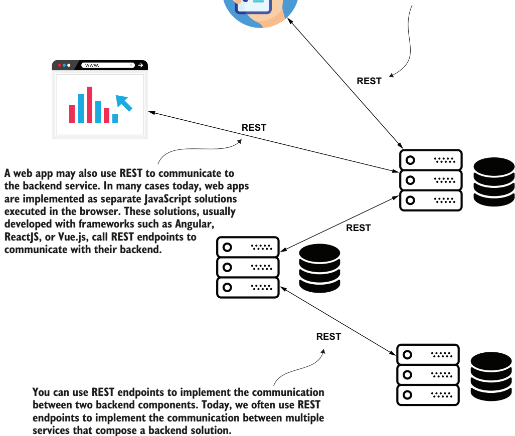
Figure 10.1 REST services are a communication method between two apps. Today, you can find REST services in many places. A web client app or mobile app may call its backend solution through REST endpoints, but even backend services might communicate using REST web service calls.
