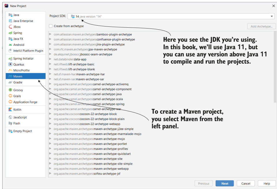
Figure 2.1 Creating a new Maven project. After going to File > New > Project, you get to this window, where you need to select the type of the project from the left panel. In our case, we choose Maven. In the upper part of the window, you select the JDK you wish to use to compile and run the project.
