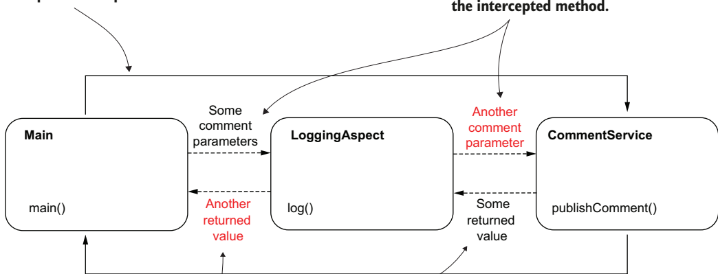
Figure 6.11 An aspect can change the parameters used to call the intercepted method and the returned value received by the intercepted method's caller. This approach is powerful, and it gives flexible control of the intercepted method.
