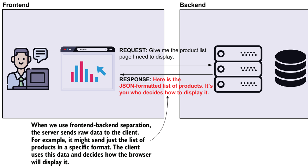
Figure 7.5 Using frontend-backend separation. The server doesn't respond with the exact data that needs to be displayed by the browser. The backend sends the data to the client but doesn't tell the browser how to display this data or what to do with it. The backend now only sends raw data (usually in an easily parsable format like JSON or XML). The browser executes a frontend app that takes the server's raw response and processes it to display the data.
