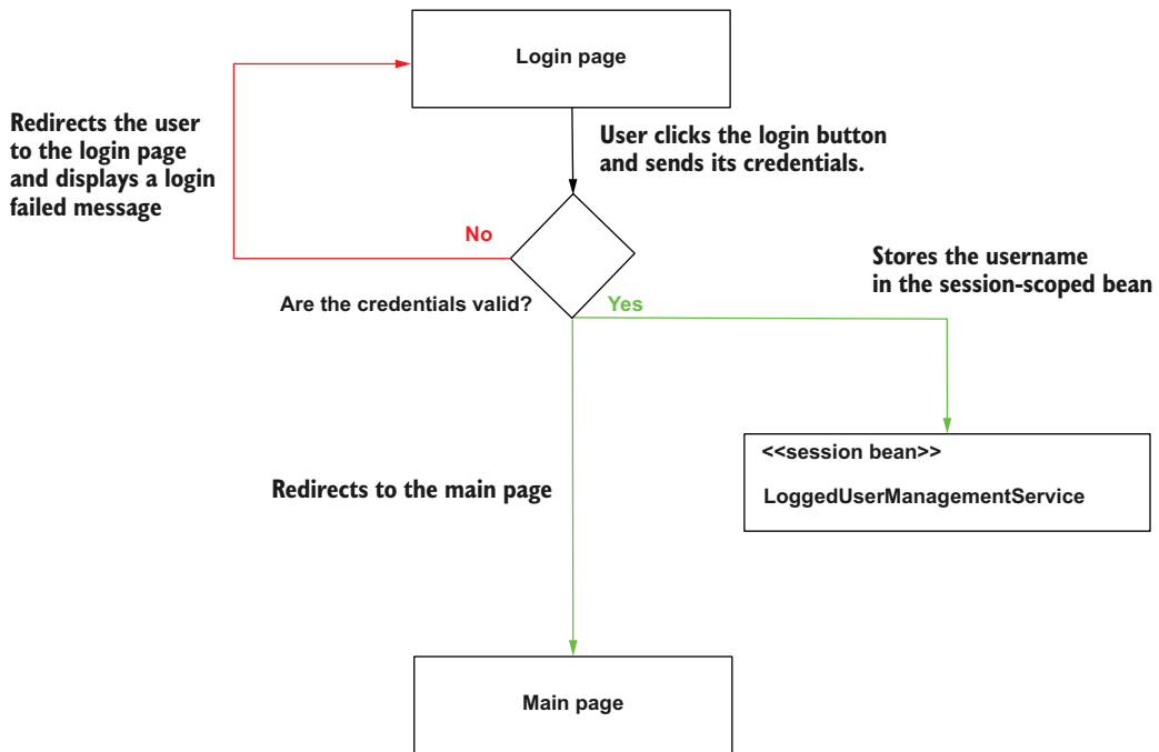
Figure 9.11 The login flow implemented in the example. When the user submits their credentials, the login process begins. If the user's credentials are correct, the username is stored in the session-scoped bean, and the app redirects the user to the main page. If the credentials are not valid, the app redirects the user back to the login page and displays a failed login message.
