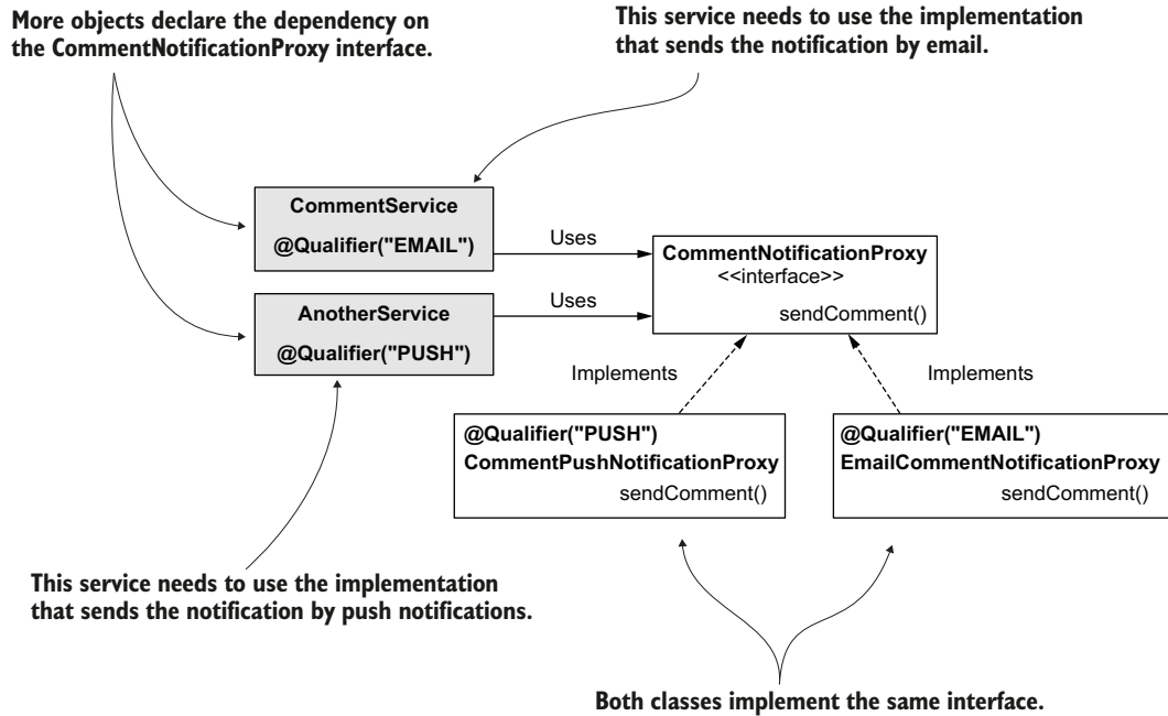
Figure 4.11 If different objects need to use different implementations of the same contract, we can use @Qualifier to name them and tell Spring where and what it needs to inject.
