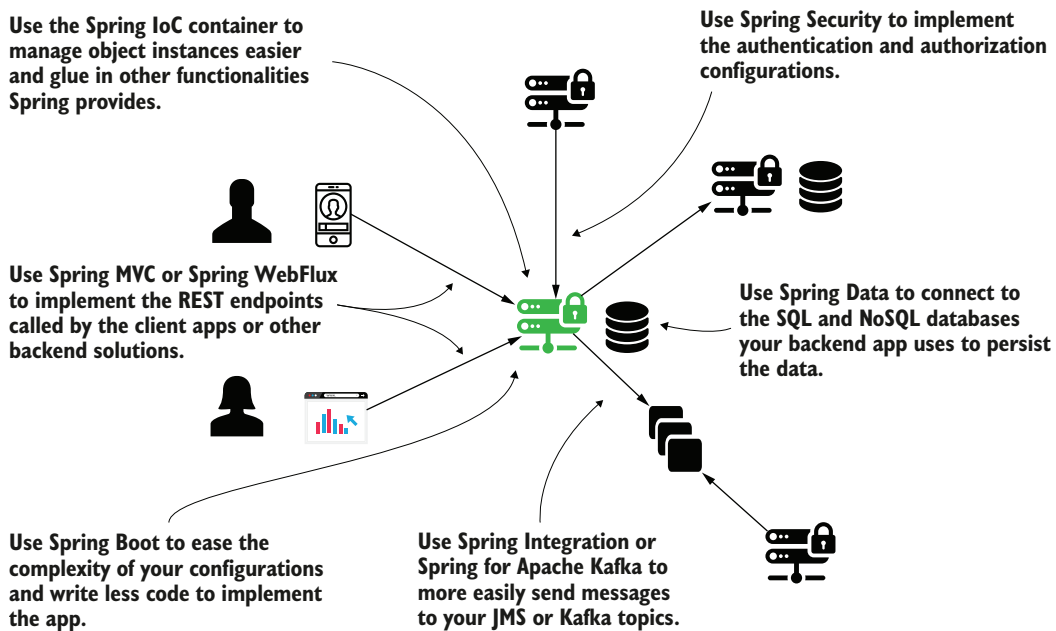
Figure 2 The possibilities of using Spring in a backend application are nearly endless, and include exposing functionalities that other applications can call, managing the database access, securing the application, and managing integration through third-party message brokers.
