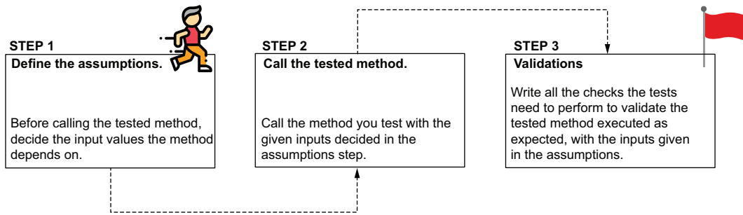
Figure 15.5 The steps for writing a unit test. Write the assumptions by defining the method inputs. Call the method with the defined assumptions and write the checks the tests need to perform to validate the method's behavior is correct.
