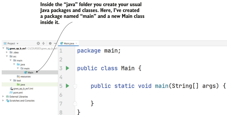
Figure 2.4 Inside the "java" folder, you create the usual Java packages and classes of your application. These are the classes that define the whole logic of your app and make use of the dependencies you provide.
