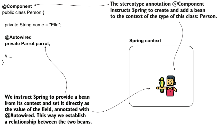
Figure 3.9 Using the @Autowired annotation over the field, we instruct Spring to provide a value for that field from its context. Spring creates the two beans, person and parrot, and injects the parrot object to the field of the bean of type Person.
