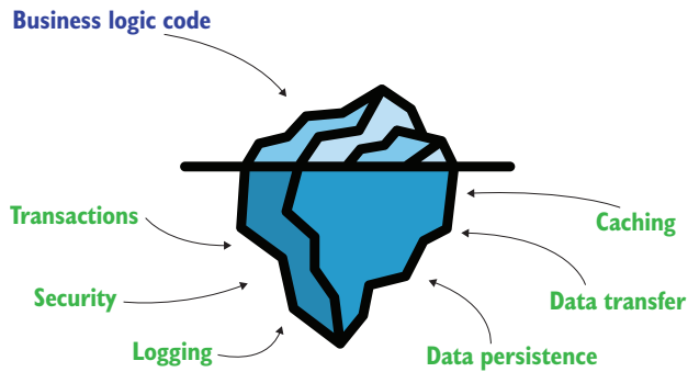
Figure 1 The user's perspective is similar to viewing an iceberg. Users mainly observe the results of the business logic code, but this is only a small part of what builds the app's complete functionality. Like an iceberg that is mostly underwater and hidden from view, we don't see most of the code in an enterprise app because it's provided by dependencies.
