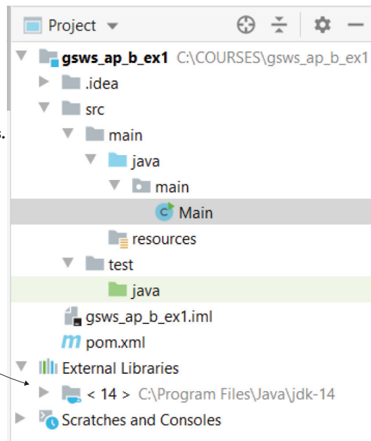
Figure 2.5 With a default pom.xml file, your project only uses the JDK as an external dependency. One of the reasons you change the pom.xml file (and the one we'll use in this book) is to add new dependencies your app needs.
