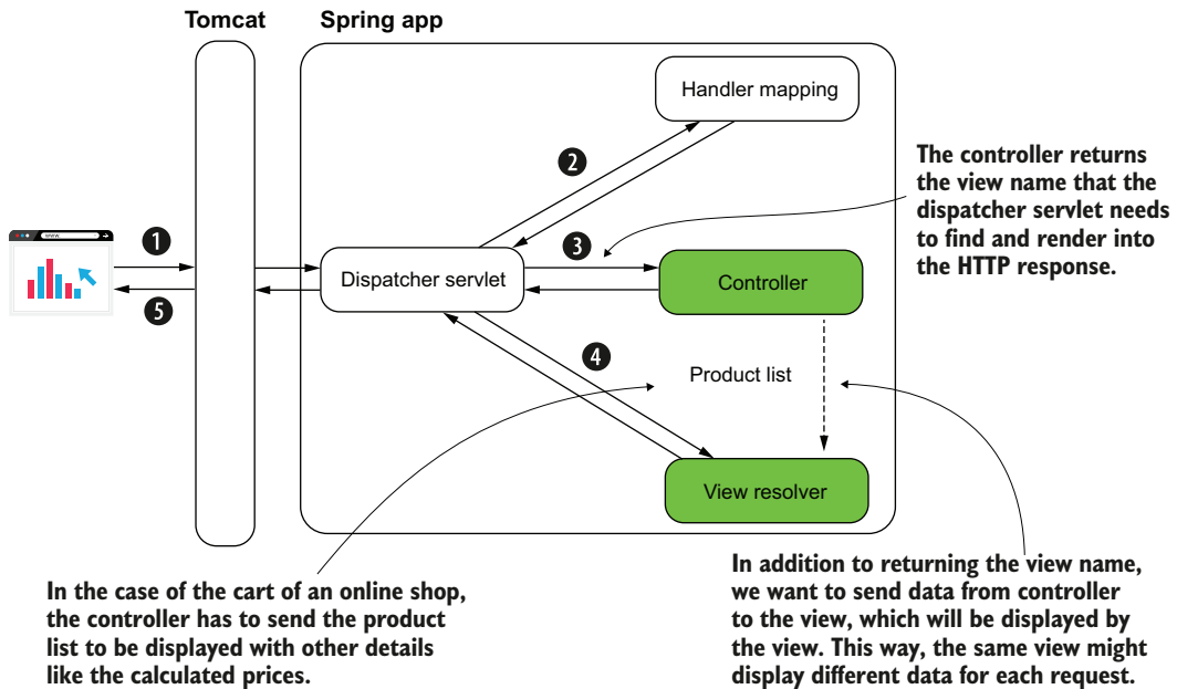
Figure 8.3 The Spring MVC flow. To define a dynamic view, the controller needs to send data to the view. The data the controller sends can be different for each request. For example, in an online shop's cart functionality, the controller initially sends a list of one product to the view. After the user adds more products, the list the controller sends contains all the products in the cart. The same view shows different information for these requests.
