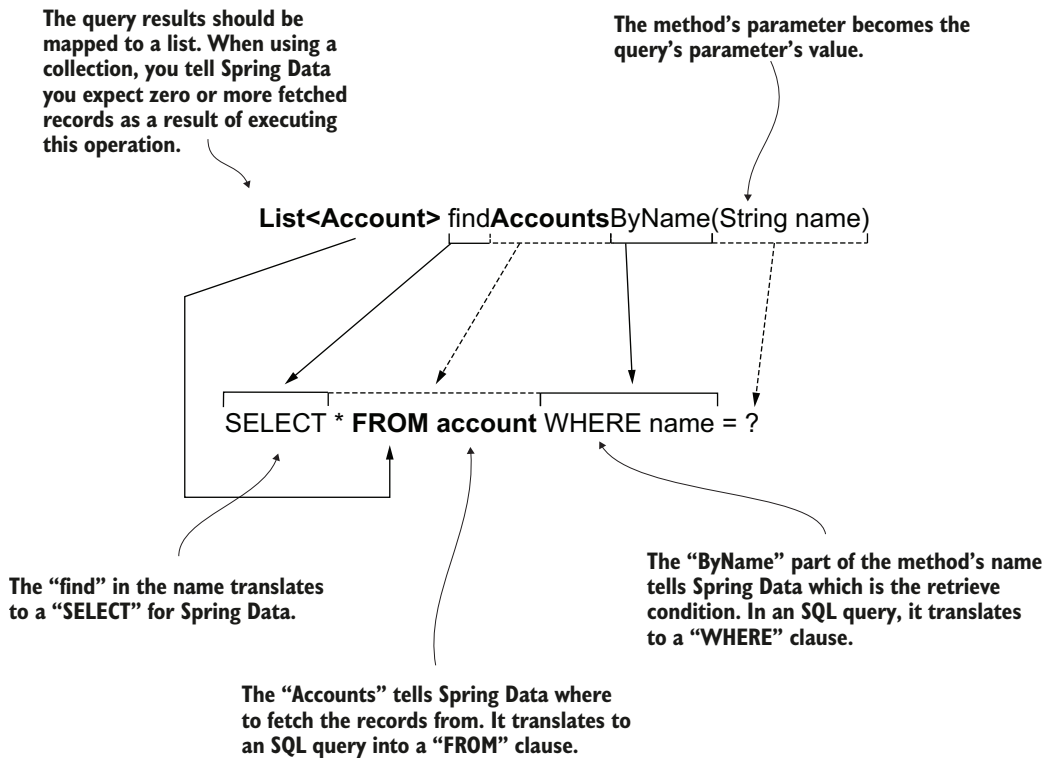
Figure 14.12 The relationship between the repository’s method name and the query Spring Data creates behind the scenes
