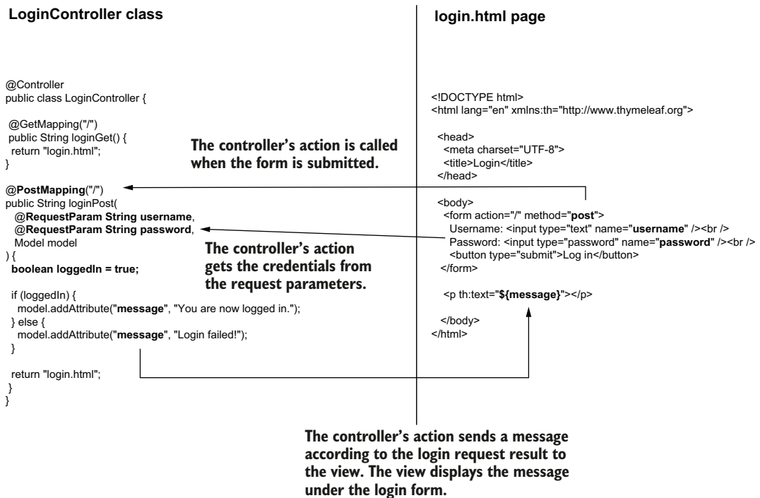
Figure 9.5 The dispatcher servlet calls the controller's action when someone submits the HTML login form. The controller's action gets the credentials from the HTTP request parameters. According to the login result, the controller sends a message to the view, and the view displays this message under the HTML form.
