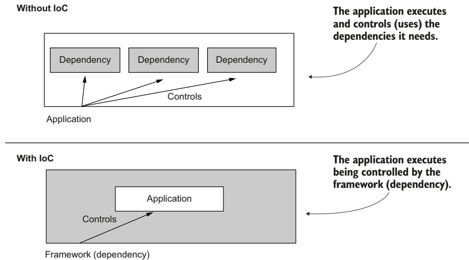
Figure 1.4 Inversion of control. Instead of executing its own code, which makes use of several other dependencies, in case of an IoC scenario, the app execution is controlled by the dependency. The Spring framework controls an app during its execution. Therefore, it implements an IoC scenario of execution.
