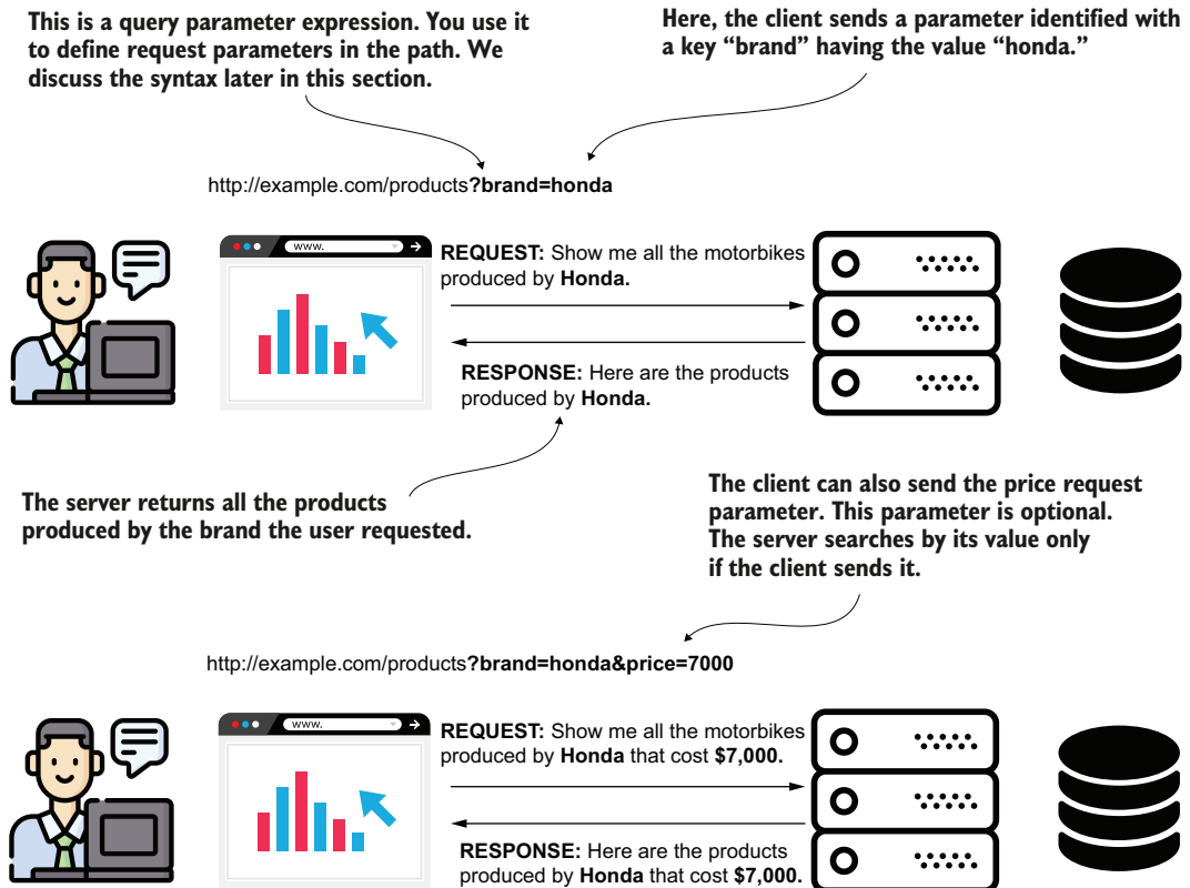
Figure 8.5 A request parameter can be optional. A common scenario for using request parameters is implementing a search functionality where the search criteria are optional. The client sends only some of the request parameters, and the server knows to use only the values it receives. You implement the server to consider it might not get values for some of the parameters.
