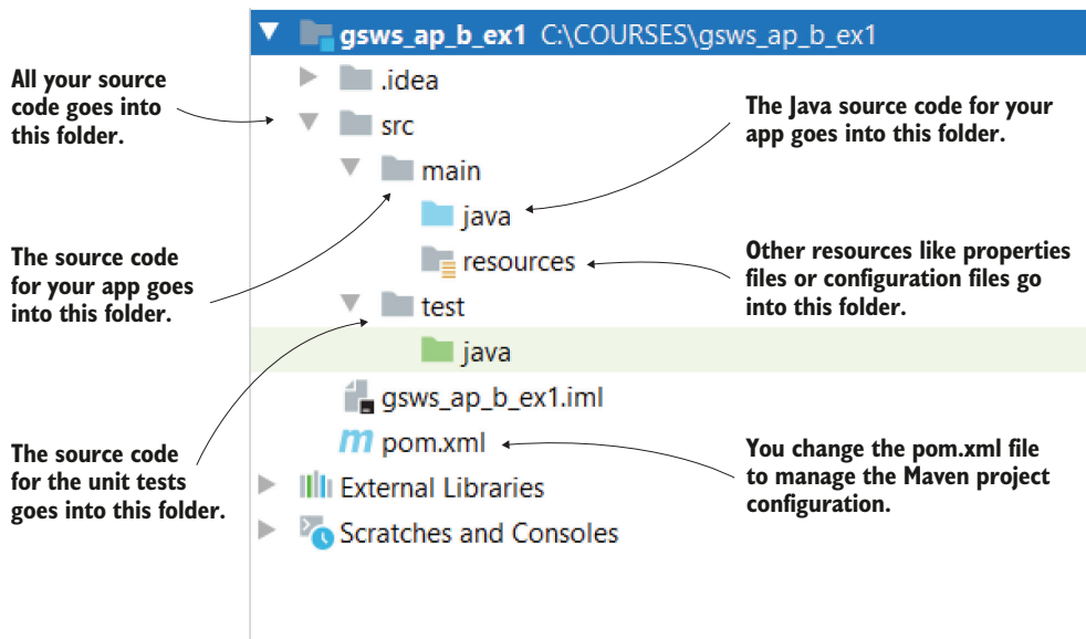
Figure 2.3 How a Maven project is organized. Inside the src folder, we add everything that belongs to the app: the application's source code goes into the main folder, and the source code for the unit tests goes into the test folder. In the pom.xml file we write configurations for the Maven project (in our examples we'll primarily use it to define the dependencies).
