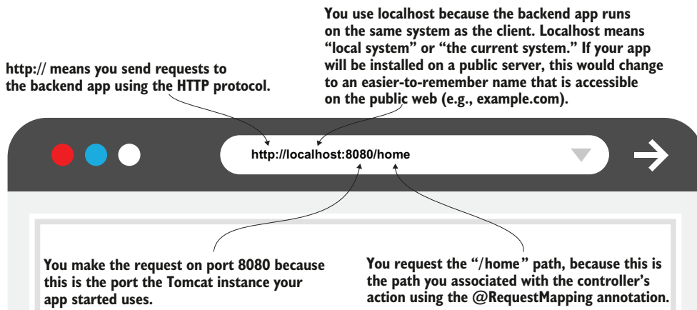
Figure 7.16 Testing the implementation. Using a browser, send a request to the backend app. You need to use the port Tomcat opened and the path you specified with the @RequestMapping annotation.
