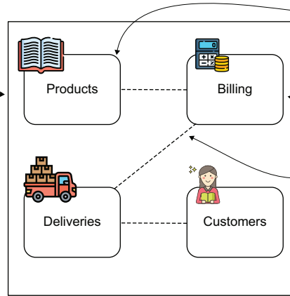
Figure A.1 A monolithic application. The application implements all the functionalities in just one process. The implementations interact with one another inside the process to develop the business flow.
