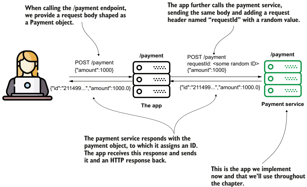
Figure 11.3 The payment service exposes an endpoint that requires an HTTP request body. The app uses OpenFeign , RestTemplate , or WebClient to send requests to the endpoint the payment service exposes.
