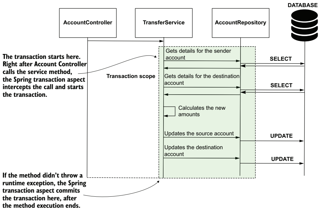
Figure 13.7 The transaction starts just before the service method execution and ends just after the method successfully ended. If the method doesn't throw any runtime exception, the app commits the transaction. If any step causes a runtime exception, the app restores the data to how it was before the transaction started.
