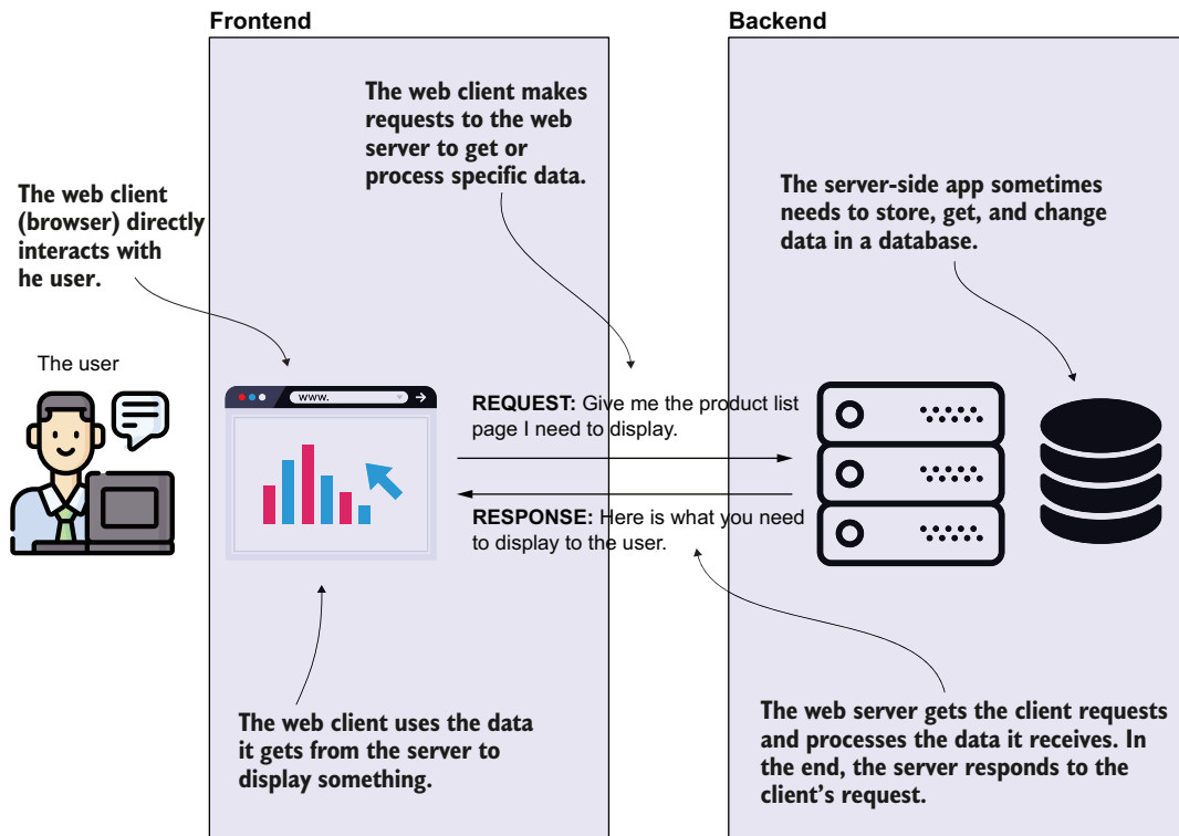
Figure 7.2 The big picture of a web app. The user interacts with the app through its frontend. The frontend communicates with the backend to execute logic at the user's request and get the data to display. The backend executes business logic and sometimes persists data in a database or communicates with other external services.
