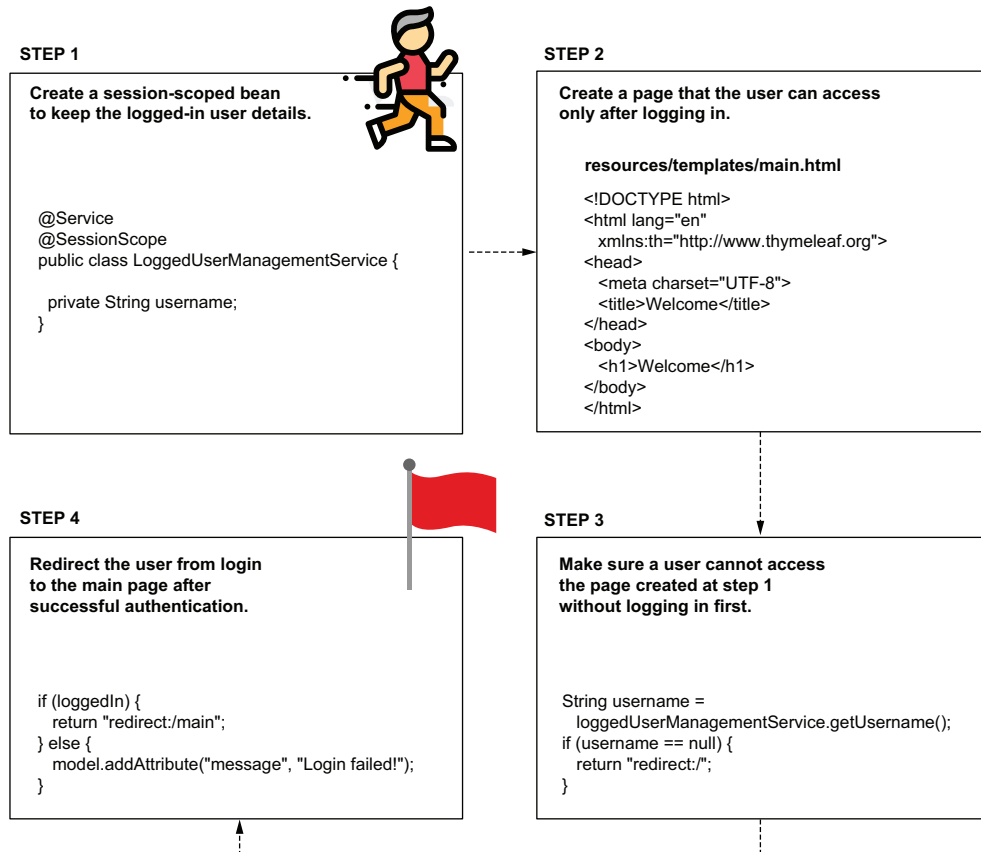
Figure 9.10 We use a session-bean to implement a section of the app that only a logged-in user can access. Once the user authenticates, the app redirects them to a page they can only access once authenticated. If the user tries to access this page before authentication, the app redirects them to the login form.
