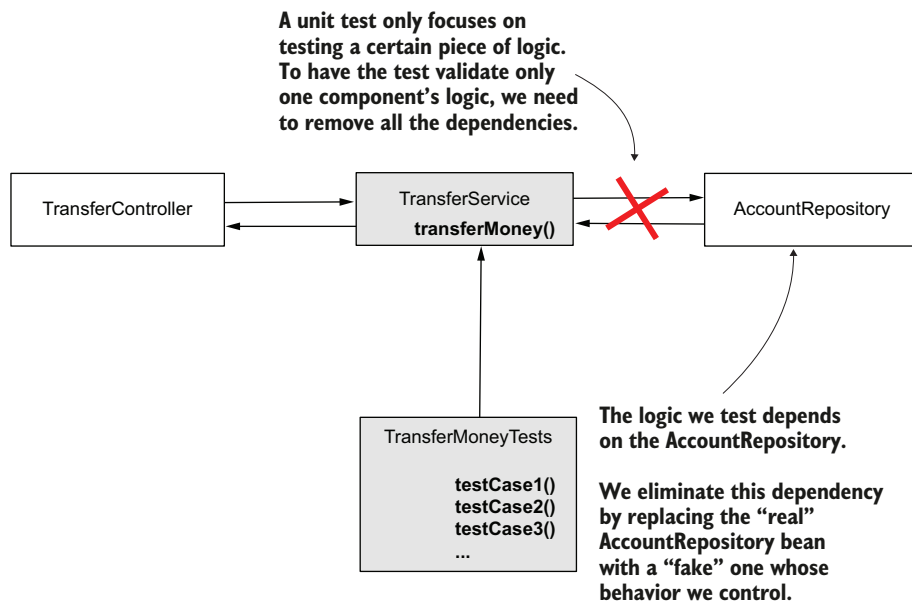
Figure 15.7 To allow the unit test to focus only on the transferMoney() method's logic, we eliminate the dependency to the AccountRepository object. We use a mock object to replace the real AccountRepository instance, and we control this fake instance to test how the transferMoney() method behaves in different situations.
