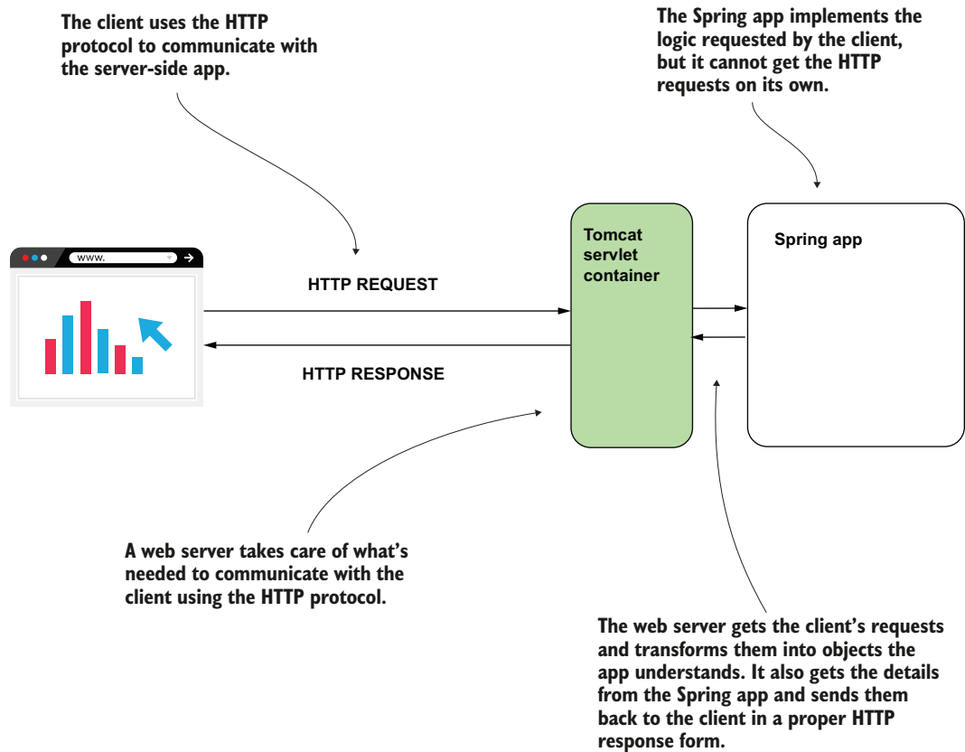
Figure 7.6 A servlet container (e.g., Tomcat) speaks HTTP. It translates the HTTP request to our Spring app and the app's response into an HTTP response. This way, we don't need to care about the protocol used for communication on the network, as we simply write everything as Java objects and methods.
