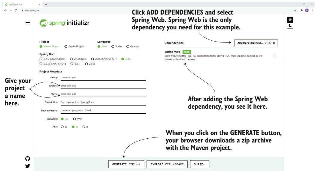
Figure 7.12 For our example, we need to add the Spring Web dependency. You can add it using the Add Dependencies button on the right upper-hand side of the window. You also need to give a name to your project.
