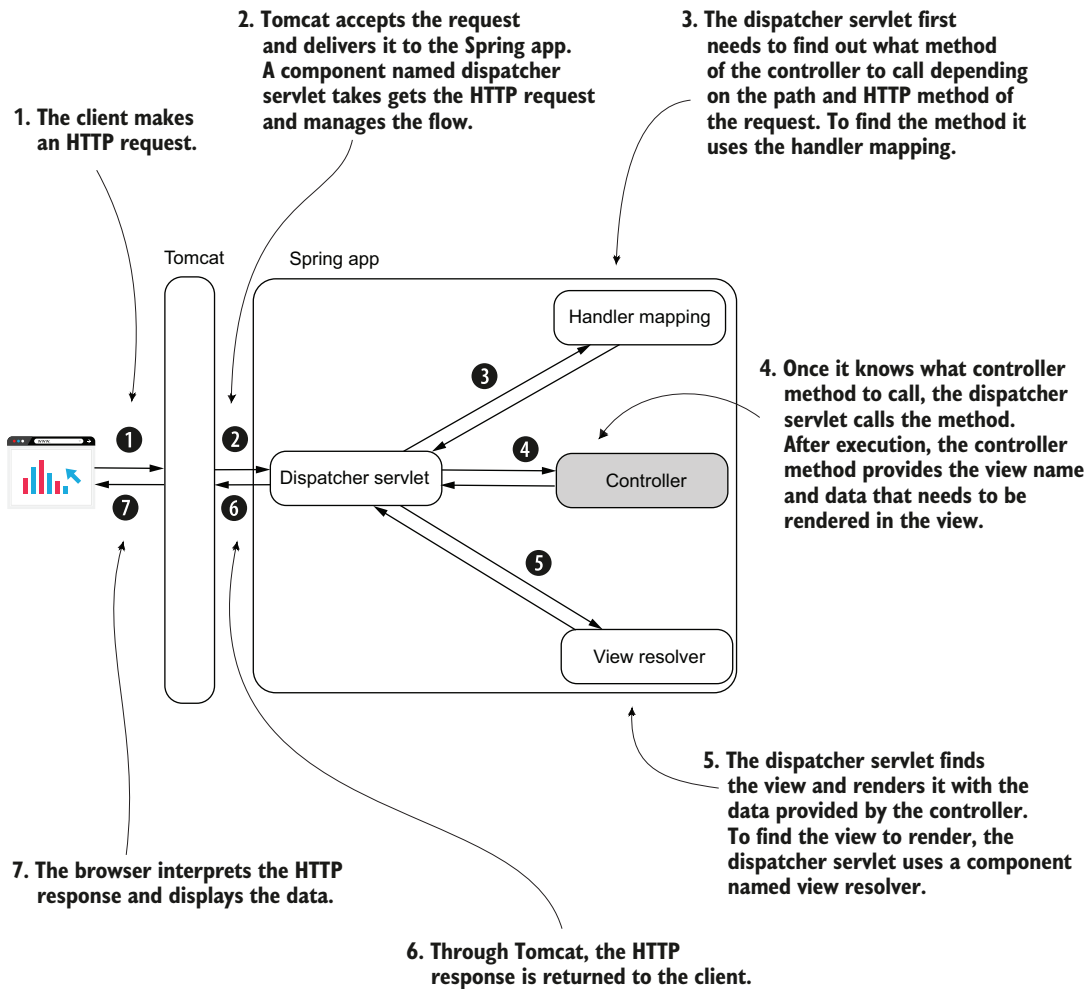
Figure 7.18 The Spring MVC architecture. In the diagram, you find the main components of Spring MVC. These components and the way they collaborate are responsible for a web app's behavior. The controller (shaded differently) is the only component you implement. Spring Boot configures the other components.
