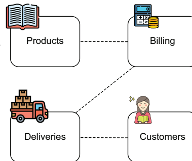
Figure A.5 In a SOA, each feature is an independent process. This way, you can decide to scale just the features that need more resources.
