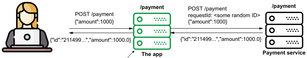
Figure 11.4 We now implement the app that consumes the /payment endpoint the payment service exposes. We use OpenFeign to implement the functionality that consumes the REST endpoint.
