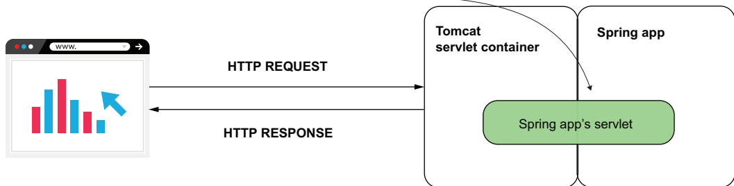
Figure 7.8 The Spring app defines a servlet object and registers it into the servlet container. Now both Spring and the servlet container know this object and can manage it. The servlet container calls this object for any client request, allowing the servlet to manage the request and the response.
