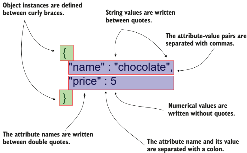
Figure D.2 Describing an object instance in JSON. We surround the attribute-value pairs with curly braces. A colon separates the attribute name and its value. The attribute-value pairs are separated with commas.
