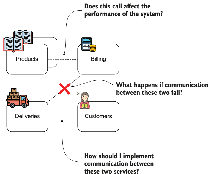
Figure A.7 Communication between services adds complexity to the system. We need to decide how to implement the communication between two services. We also need to understand what could happen if the communication fails and how to solve potential problems caused by malfunctioning communication.
