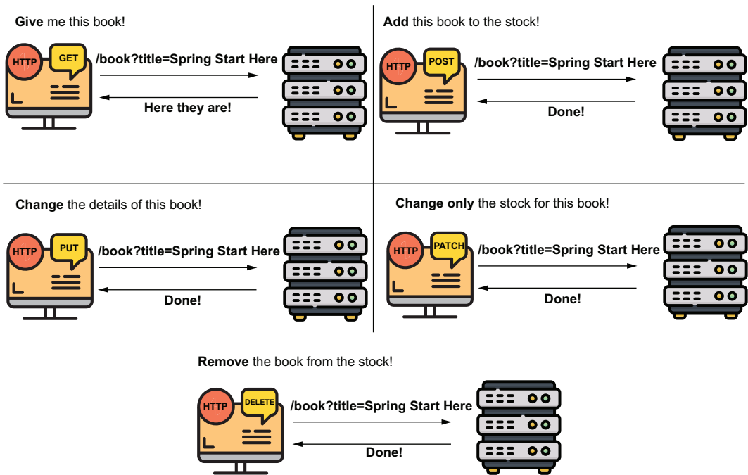
Figure 8.9 The basic HTTP methods. You use GET for retrieving data, POST for adding data, PUT for changing a record, PATCH for changing a part of the record, and DELETE to remove data. The client must use the appropriate HTTP method to express the action executed by a specific request.
