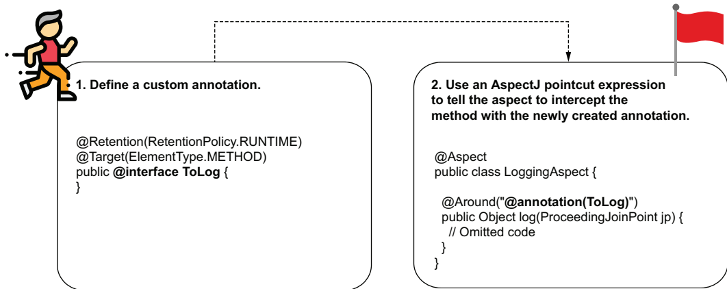
Figure 6.12 The steps for intercepted annotated methods. You need to create a custom annotation you want to use to annotate the methods your aspect needs to intercept. Then you use a different AspectJ pointcut expression to configure the aspect to intercept the methods annotated with the custom annotation you created.
