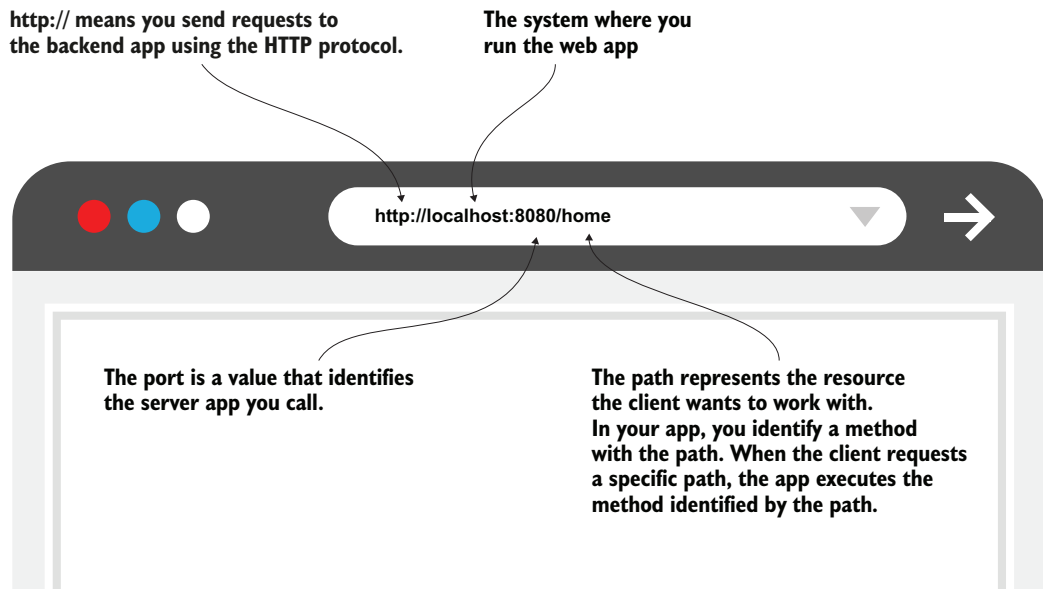
Figure C.2 The HTTP request URI identifies the resource the client requests to work with. The first part of the URI identifies the protocol and the server that runs the server app. The path identifies a resource exposed by the server.
