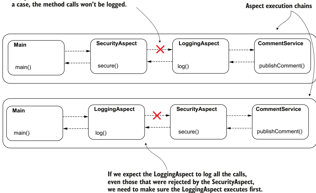
Figure 6.14 The aspect execution order matters. Depending on your app's requirements, you need to choose a specific order for the aspects to execute. In this scenario, the LoggingAspect cannot log all the method executions if the SecurityAspect executes first.
