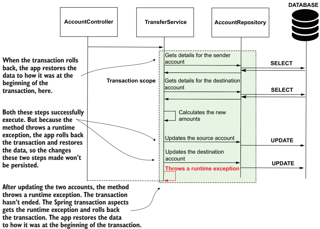
Figure 13.8 When the method throws a runtime exception, Spring rolls back the transaction. All the successful changes made on the data are not persisted. The app restores the data to how it was when the transaction started.
