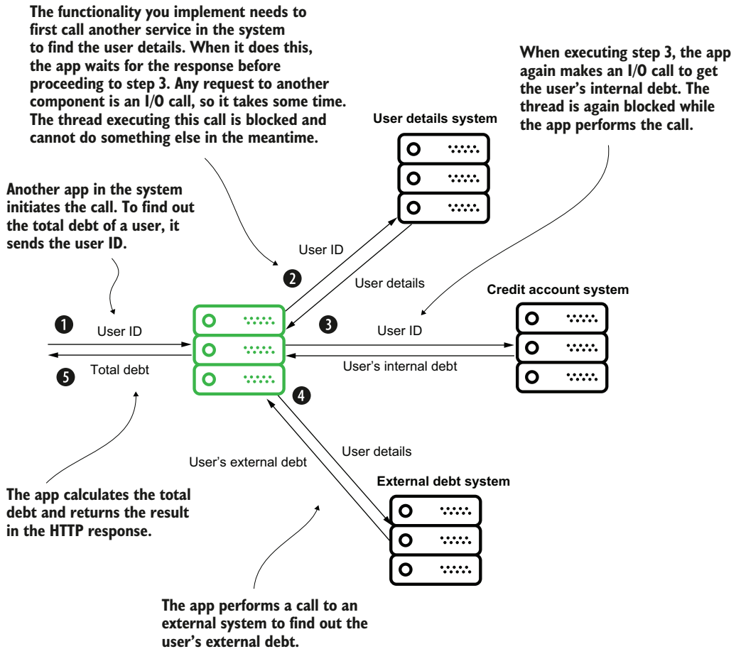
Figure 11.7 A functionality scenario for demonstrating the usefulness of a reactive approach. A banking app needs to call several other apps to calculate the total debt of a user. Due to these calls, the thread executing the request is blocked several times while waiting for I/O operations to finish.
