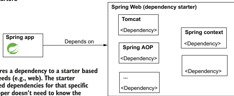
Figure 7.14 Using dependency starters. Instead of individually referring to specific dependencies, the app now depends on only a starter. The starter contains all the needed dependencies for implementing a specific capability. The starter also makes sure these dependencies are compatible with one another.
