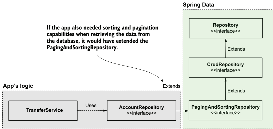
Figure 14.8 If the app needs sorting and paging capabilities, it should extend a more particular contract. The app provides a bean that implements the contract, which can then be injected from any other component that needs to use it.
