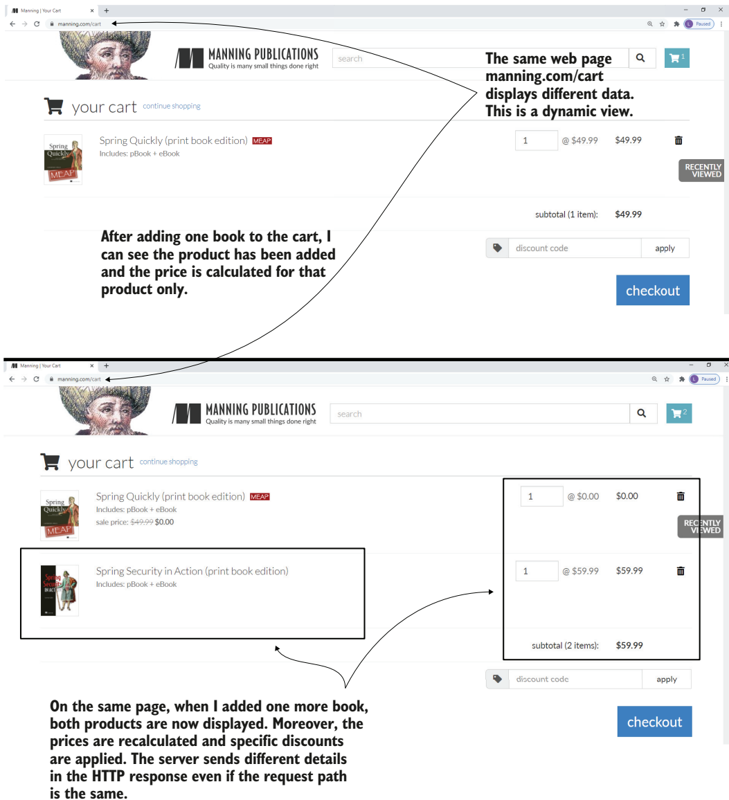
Figure 8.1 A dynamic view presented with the Manning shopping cart functionality. Even if the requested page is the same, the content of the page is different. The backend sent different data in the response before and after adding one more product to the cart.
