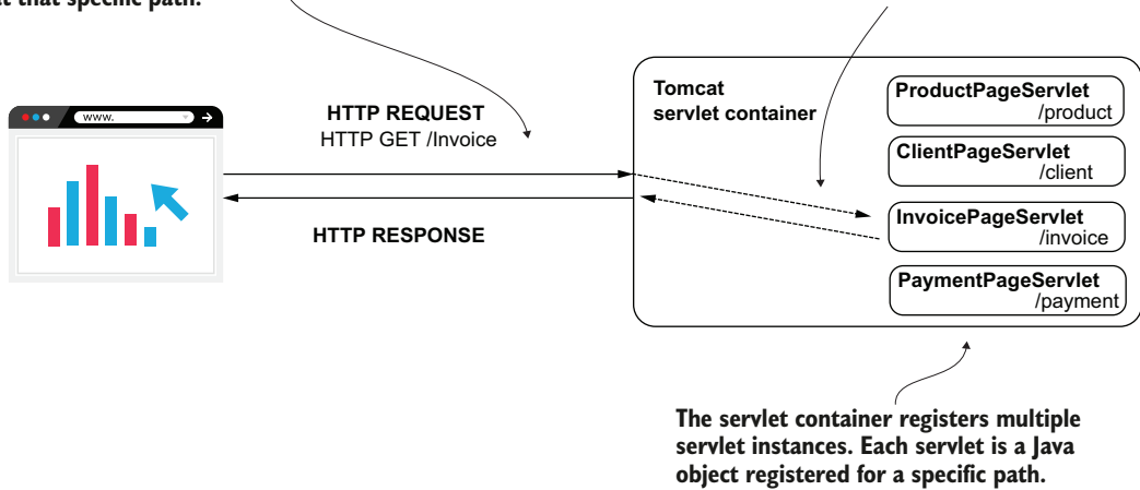
Figure 7.7 The servlet container (Tomcat) registers multiple servlet instances. Each servlet is associated with a path. When the client sends a request, Tomcat calls a method of the servlet associated with the path the client requested. The servlet gets the values on the request and builds the response that Tomcat sends back to the client.
