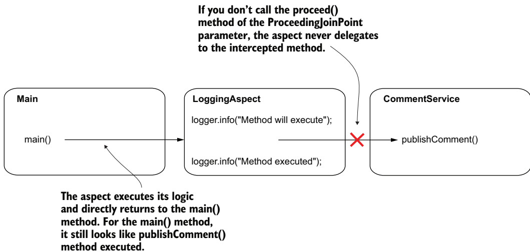
Figure 6.8 If you don't call the proceed() method of the ProceedingJoinPoint parameter of the aspect, the aspect never delegates further to the intercepted method. In this case, the aspect simply executes instead of the intercepted method. The caller of the method doesn't know that the real method is never executed.
