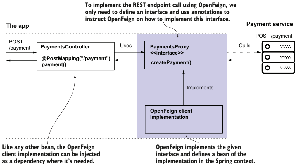
Figure 11.5 With OpenFeign, you only need to define an interface (a contract) and tell OpenFeign where to find this contract to implement it. OpenFeign implements the interface and provides the implementation as a bean in the Spring context based on configurations you define with annotations. You can inject the bean from the Spring context anywhere you need it in your app.
