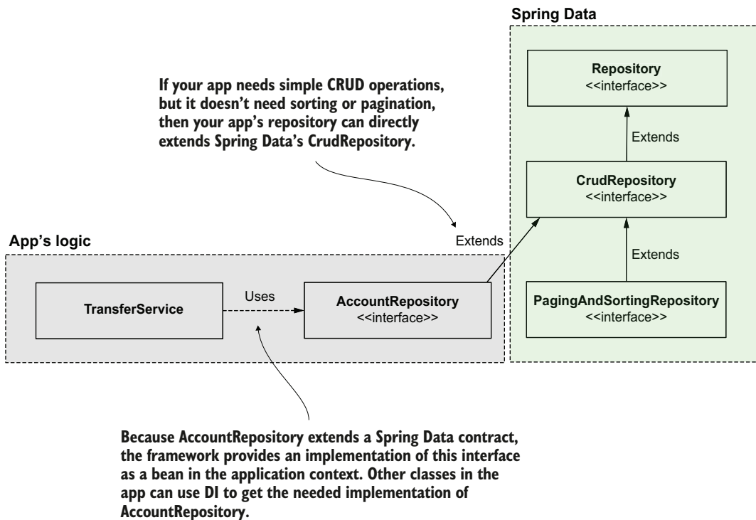
Figure 14.7 To create a Spring Data repository, you define an interface that extends one of the Spring Data contracts. For example, if your app only needs CRUD operations, the interface you define as a repository should extend the CrudRepository interface. The app adds a bean that implements the contract you define to the Spring context, so any other app components that need to use it can simply inject it from the context.
