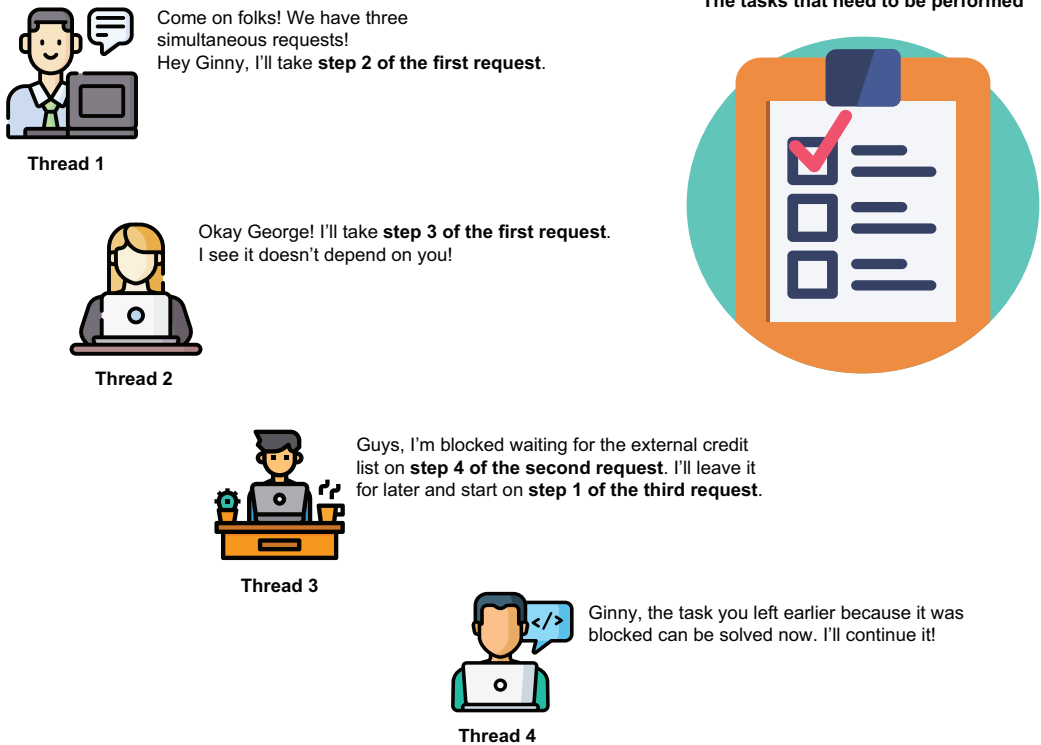
Figure 11.9 An analogy of the way a reactive app works. A thread doesn't take a request's tasks in order and wait when it's blocked. Instead, all tasks from all requests are on a backlog. Any available thread can work on tasks from any request. This way, independent tasks can be solved in parallel, and the threads don't stay idle.
