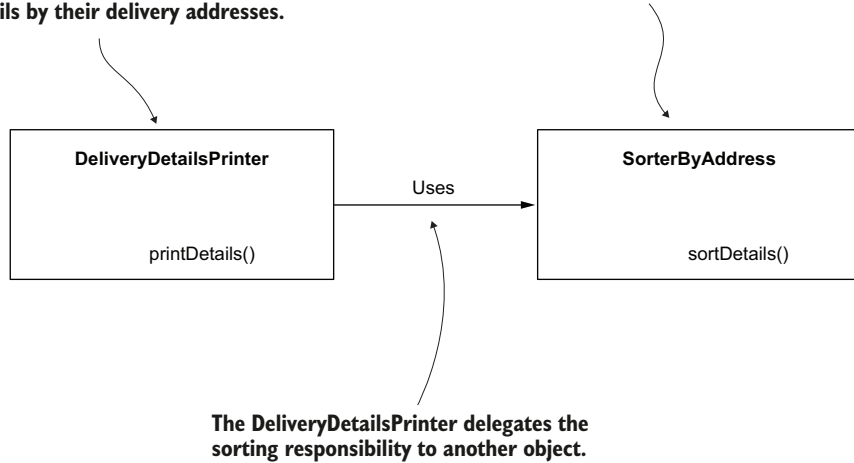
Figure 4.1 The DeliveryDetailsPrinter object delegates the responsibility of sorting the delivery details by the delivery addresses to another object named SorterByAddress .
