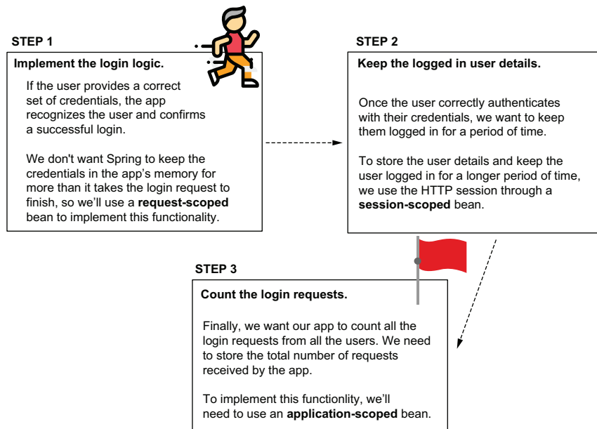
Figure 9.1 We'll implement the login functionality in three steps. For each step we implement, we'll need to use a different bean scope. In section 9.1, we'll use a request-scoped bean to implement the login logic without risking storing the credentials for longer than the login request. We'll then decide what details we need to store for the authenticated user in a session-scoped bean. Finally, we'll implement a feature to count all the login requests, and we'll use an application-scoped bean to keep the number.
