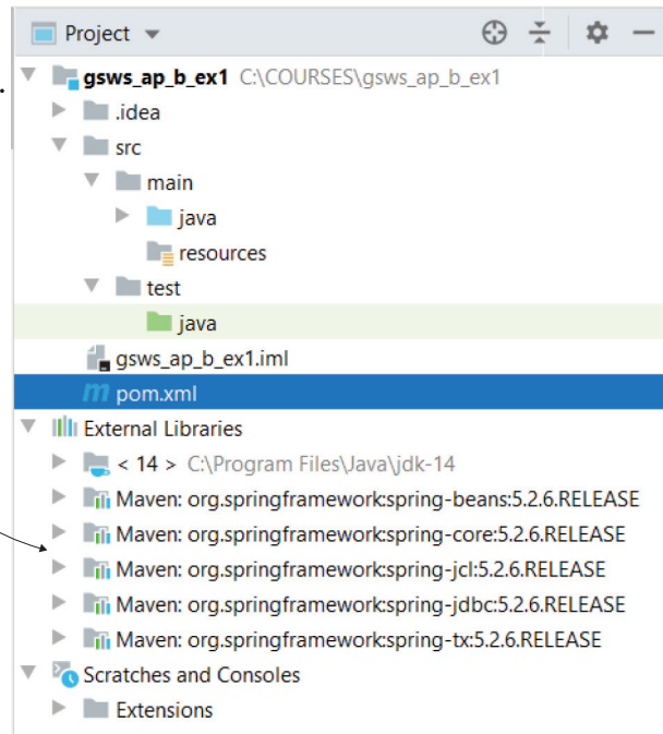
Figure 2.6 When you add a new dependency to the pom.xml file, Maven downloads the jar files representing that dependency. You find these jar files in the External Libraries folder of the project.
