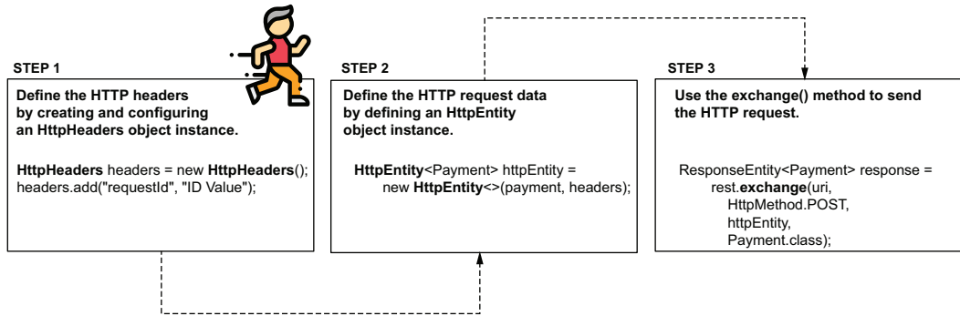
Figure 11.6 To define a more complex HTTP request, you have to use the HttpHeaders class to define the headers, then the HttpEntity class to represent the full request data. Once you defined the data on the request, you call the exchange() method to send it.
