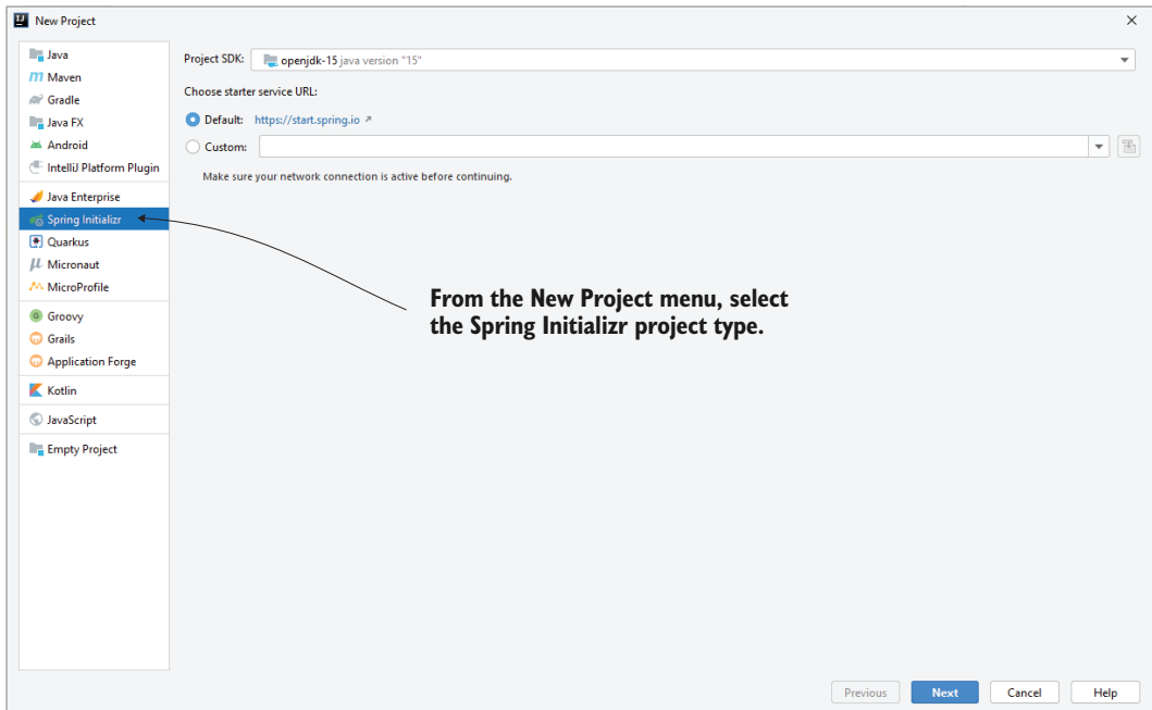
Figure 7.9 Some IDEs integrate with a project initializer service directly. For example, in IntelliJ Ultimate, you can select Spring Initializr from the New Project menu to create a Spring Boot app with a project initializer service.
