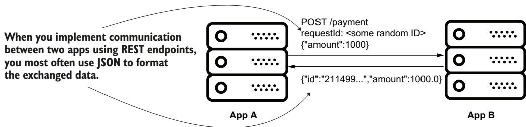
Figure D.1 When you implement business logic, it sometimes implies establishing communication between multiple apps. Most often, you use JSON to format the data the apps exchange. To implement and test your REST endpoints, you need to understand JSON.
