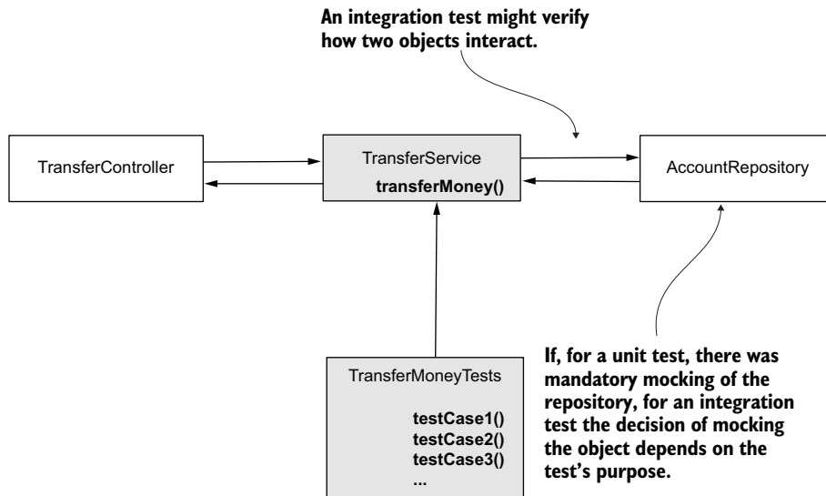
Figure 15.11 In a unit test's case, all the dependencies needed to be mocked. If the integration test's purpose is to verify how the TransferService and AccountRepository interact, the repository can be the real object. An integration test can still mock an object if its purpose doesn't verify the integration with a specific component.
