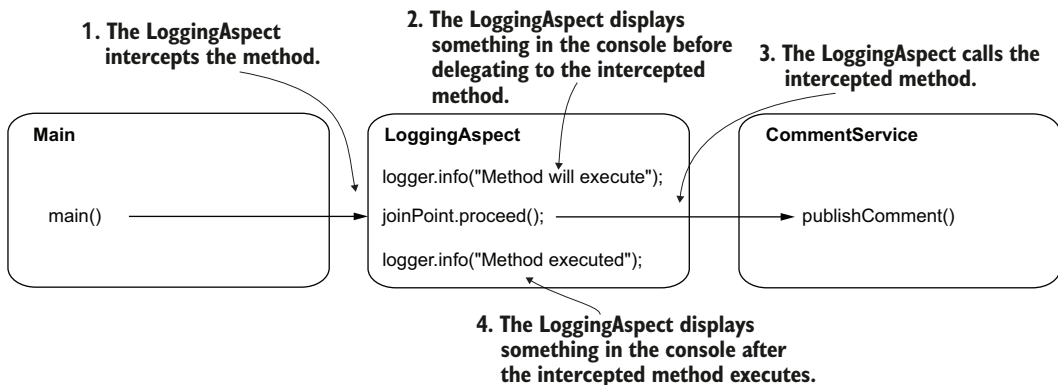
Figure 6.7 The aspect behavior. LoggingAspect wraps the method execution by displaying something before and after the method call. This way, you observe a simple implementation of an aspect.
