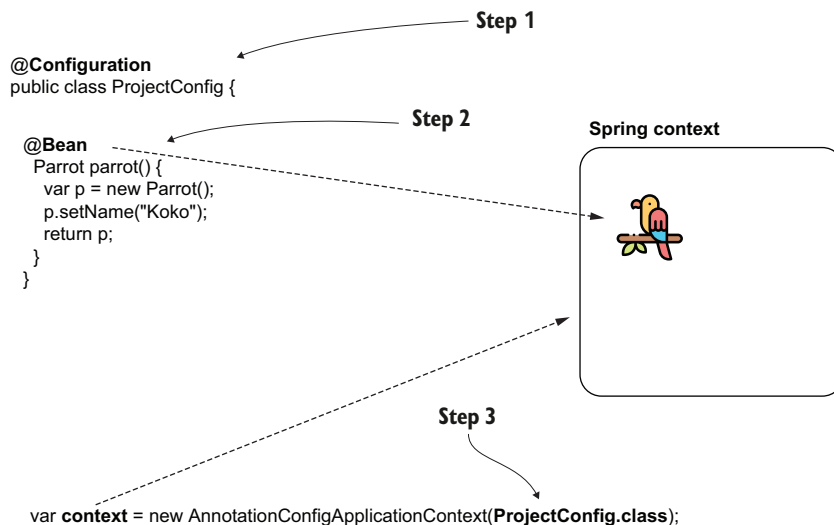
Figure 2.9 Steps for adding the bean to the context using the @Bean annotation. By adding the instance to the Spring context, you make the framework aware of the object, enabling it to manage the instance.
