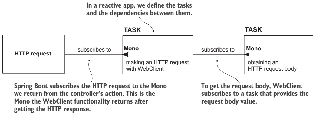
Figure 11.11 The tasks chain in a reactive app. When building a reactive web app, we define the tasks and the dependencies between them. The WebFlux functionality initiating the HTTP request subscribes to the task we create through the producer the controller's action returns. In our case, this producer is the one we get by sending the HTTP request with WebClient . For WebClient to make the request, it subscribes to another task that provides the request body.
