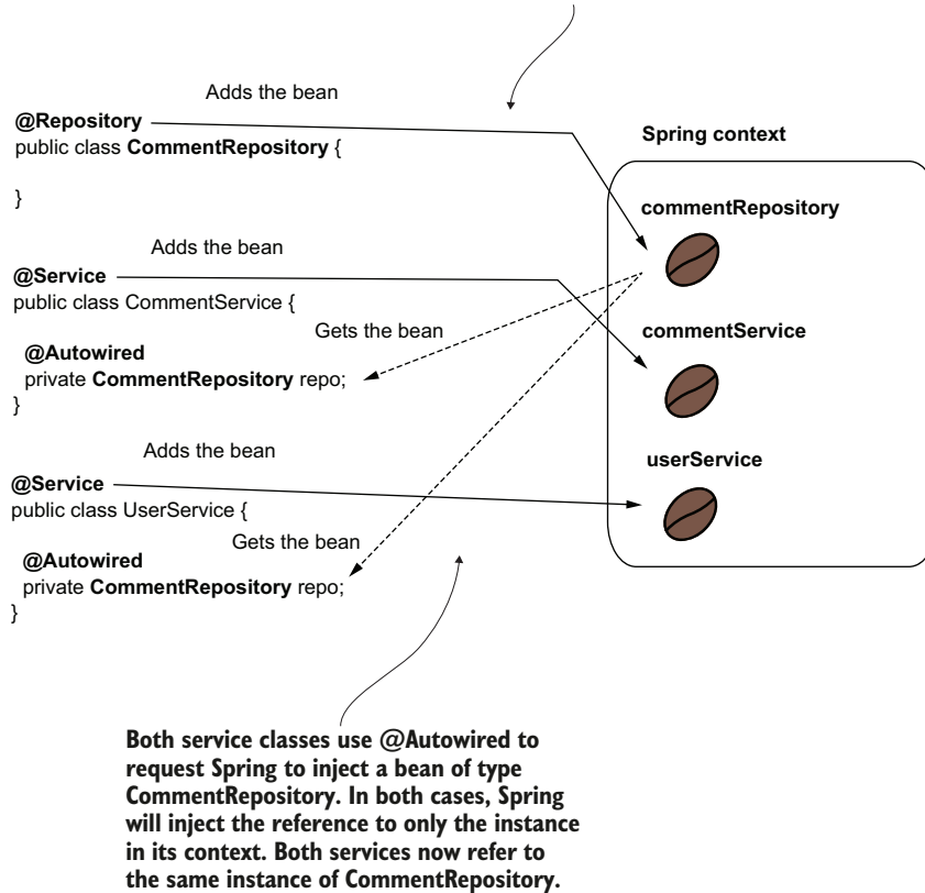
Figure 5.4 The beans are also singleton-scoped when using stereotype annotations to create them. When using @Autowired to request Spring to inject a bean reference, the framework injects the reference to the singleton bean in all the requested places.
