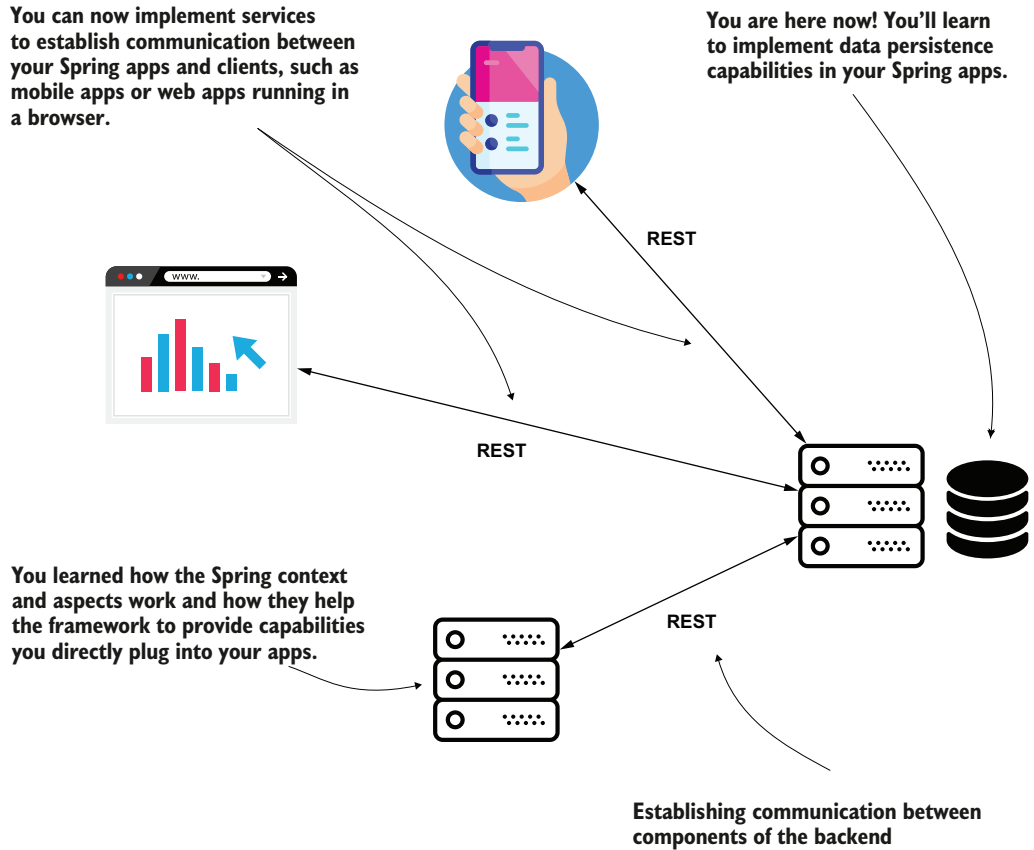
Figure 12.1 You already understand the essential parts you implement with Spring in a system. In chapters 1 through 6, you learned the fundamentals and what makes Spring able to provide the capabilities you use in your apps. In chapters 7 through 11, you learned to implement web apps and REST endpoints to establish communication between the system's components. You now start your journey in learning the valuable skills of making your Spring app work with persisted data.
