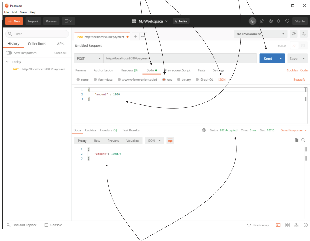
Figure 10.11 Using Postman to call the endpoint and specify the request body. You need to fill the JSON-formatted request body in the request body text area and select the data encoding as JSON . Once the request completes, Postman displays the response details.
