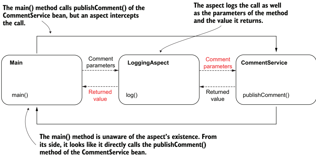
Figure 6.10 The aspect intercepts the method call, so it can access the parameters and the value returned by the intercepted method after execution. For the main() method, it looks like it directly calls the publishComment() method of the CommentService bean. The caller isn't aware that an aspect intercepted the call.
