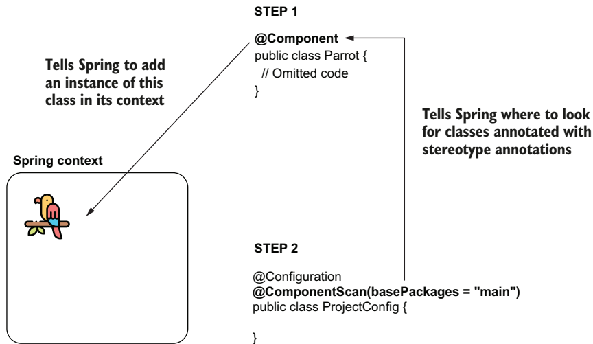
Figure 2.12 When using stereotype annotations, consider two steps. First, use the stereotype annotation ( @Component ) to annotate the class for which you want Spring to add a bean to its context. Second, use the @ComponentScan annotation to tell Spring where to look for classes annotated with stereotype annotations.
