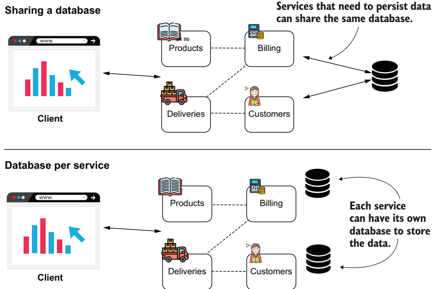
Figure A.10 In a SOA, you can decide that more services share the same database or have an individual database per service. Having various alternatives, each with its benefits and drawbacks, makes the persistence layer's design in SOA more difficult.
