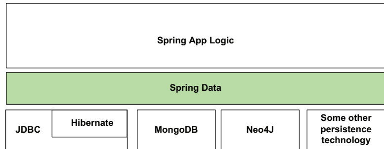
Figure 14.4 Spring Data simplifies the persistence layer implementation by offering a common set of abstractions for various technologies.
