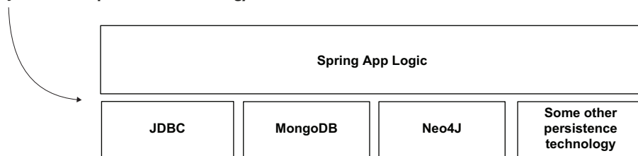
Figure 14.2 Using JDBC to connect to a relational DBMS is not the only choice for implementing an app’s persistence layer. In real-world scenarios, you’ll use other choices as well, and each way to persist data has its own library and set of APIs you need to learn to use. This variety adds a lot of complexity.
