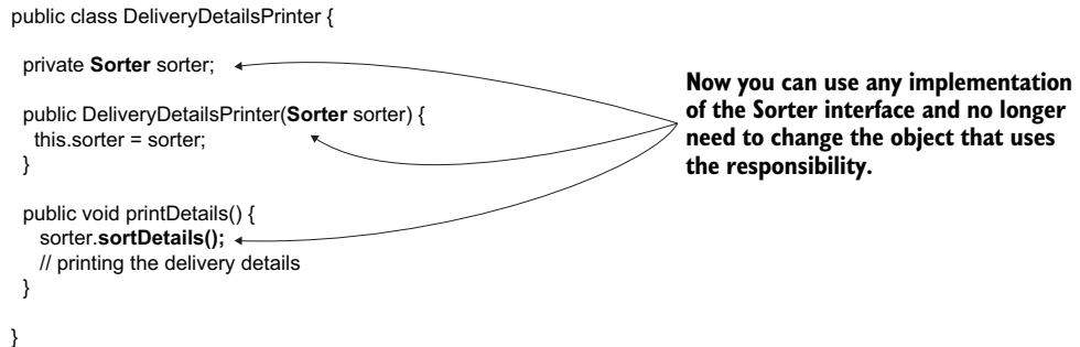
Figure 4.4 The DeliveryDetailsPrinter object depends on the Sorter interface. You can change the implementation of the Sorter interface and avoid making more changes to the object using this responsibility ( DeliveryDetailsPrinter ).
