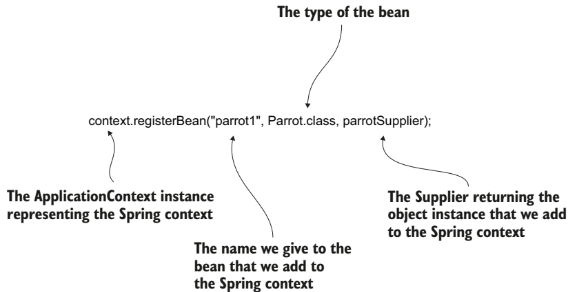
Figure 2.14 Calling the registerBean() method to add a bean to the Spring context programmatically
