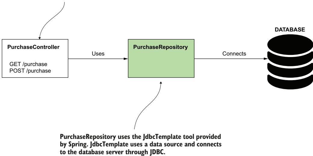
Figure 12.7 A REST controller implements two endpoints. When a client calls the endpoints, the controller delegates to a repository object to use the database.
