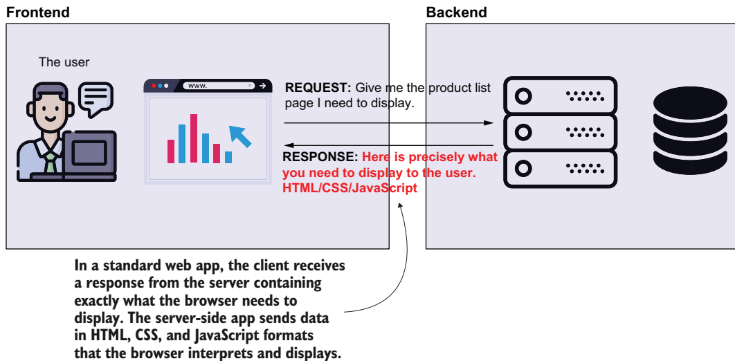
Figure 7.4 When a web app doesn't provide frontend-backend separation, the browser precisely displays what it gets from the server. The server gets requests from the browser, executes some logic, and then responds. In response, the backend provides content formatted as HTML, CSS, and other fashions that the browser interprets to display.
