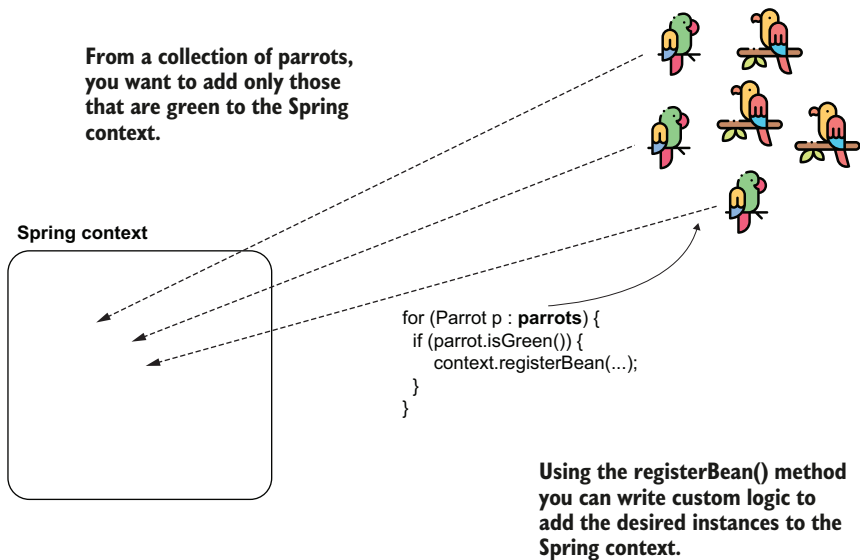
Figure 2.13 Using the registerBean() method to add specific object instances to the Spring context
