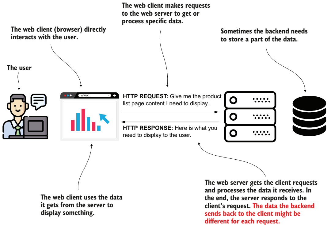
Figure 8.2 A client sends data through the HTTP request. The backend processes this data and builds a response to send back to the client. Depending on how the backend processed the data, different requests may result in other data displayed to the user.
